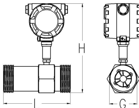
1/2 ~ 2" (DN15-DN50): Threaded connections
